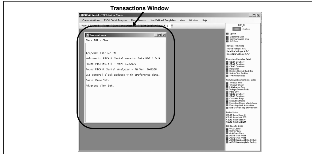
FIGURE 3-12: TRANSACTIONS WINDOW
