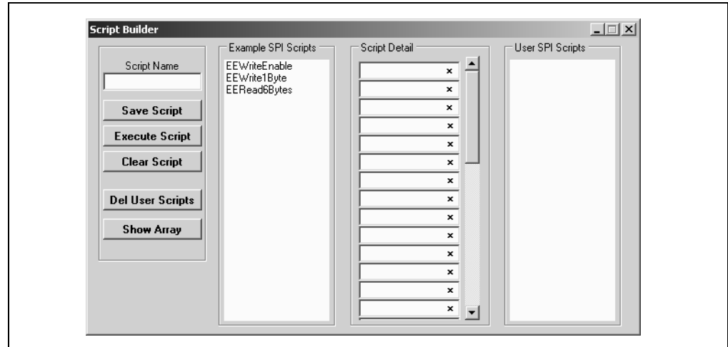
FIGURE 5-8: SPI SCRIPT BUILDER
