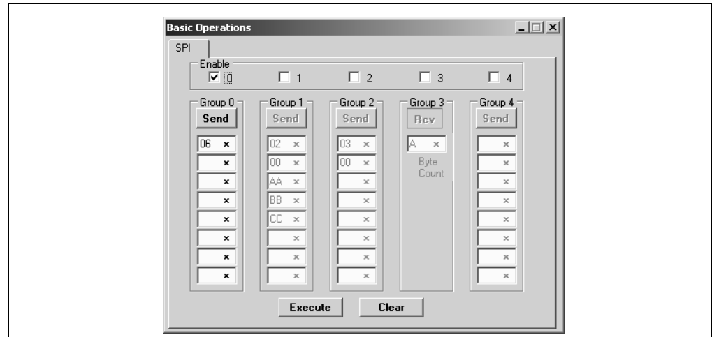
FIGURE 5-5: SEEPROM EXAMPLE – WREN COMMAND
