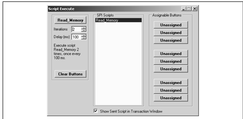
FIGURE 5-15: SPI SCRIPT EXECUTE – EXAMPLE
