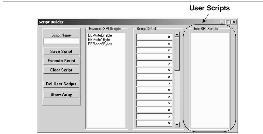
FIGURE 5-12: SPI SCRIPT BUILDER – USER SCRIPTS
