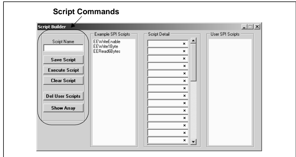
FIGURE 5-9: SPI SCRIPT BUILDER – SCRIPT COMMANDS
