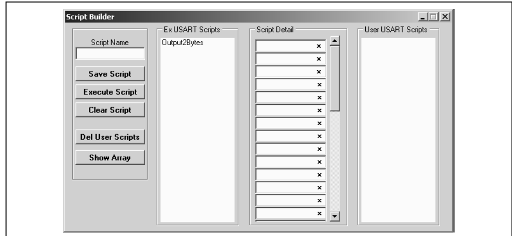
FIGURE 6-4: USART ASYNCHRONOUS SCRIPT BUILDER
