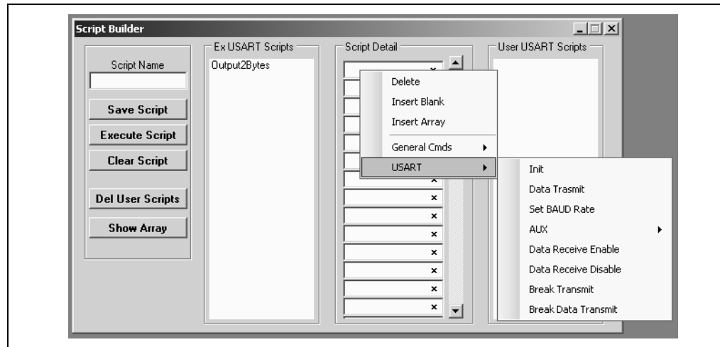
FIGURE 6-9: USART ASYNCHRONOUS SCRIPT BUILDER – CREATING A SCRIPT
